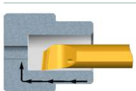
Boring
